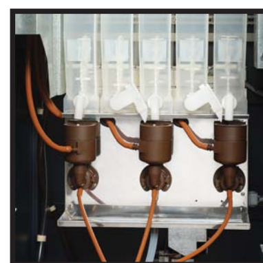
Detalle batidores S500 (Sobuble) Wippers detail S500 (Instant)
